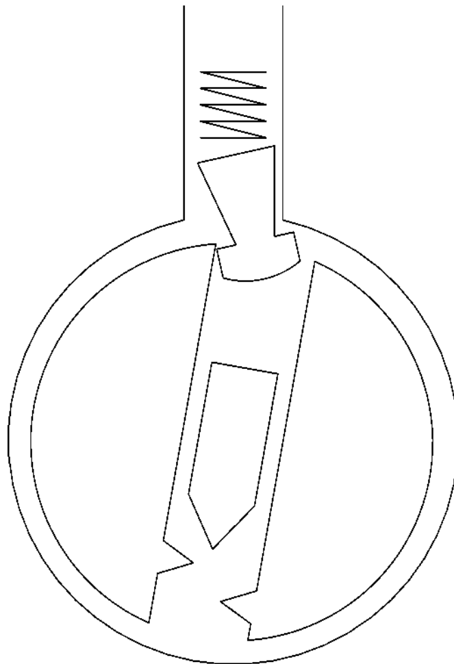
Figure 9.7: Mushroom, spool, and serrated driver pins
