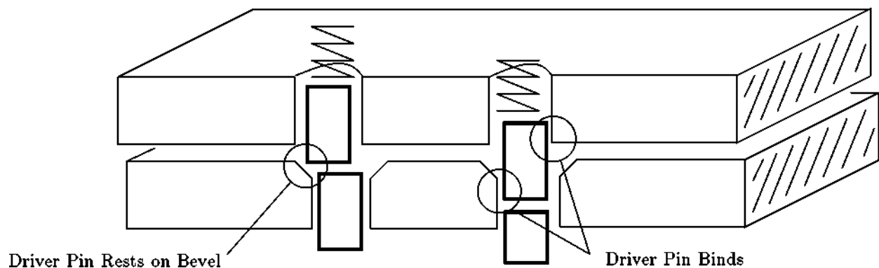
Figure 9.5: (a) Driver sets on bevel
