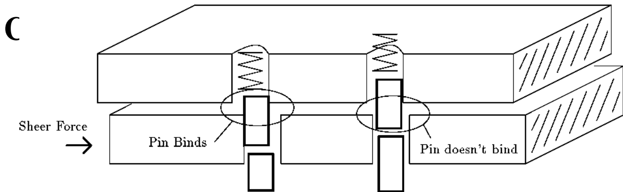
Figure 4.1: (a) Shear force causes driver to bind
