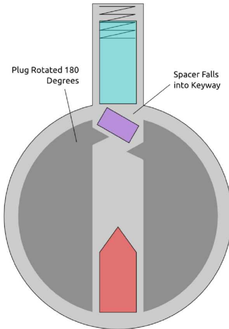
Figure 9.9: Spacer or driver can enter keyway
