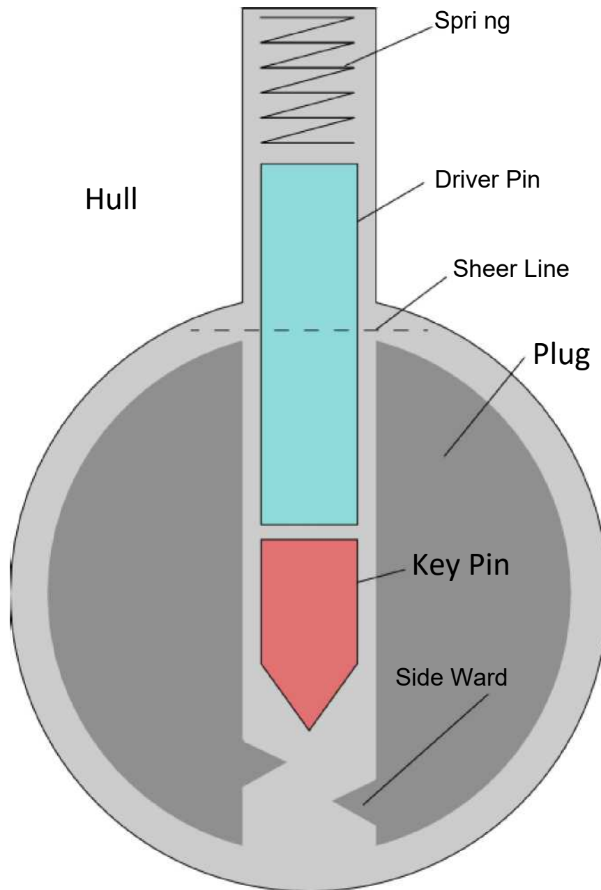
Figure 5.1: The pin-column model
