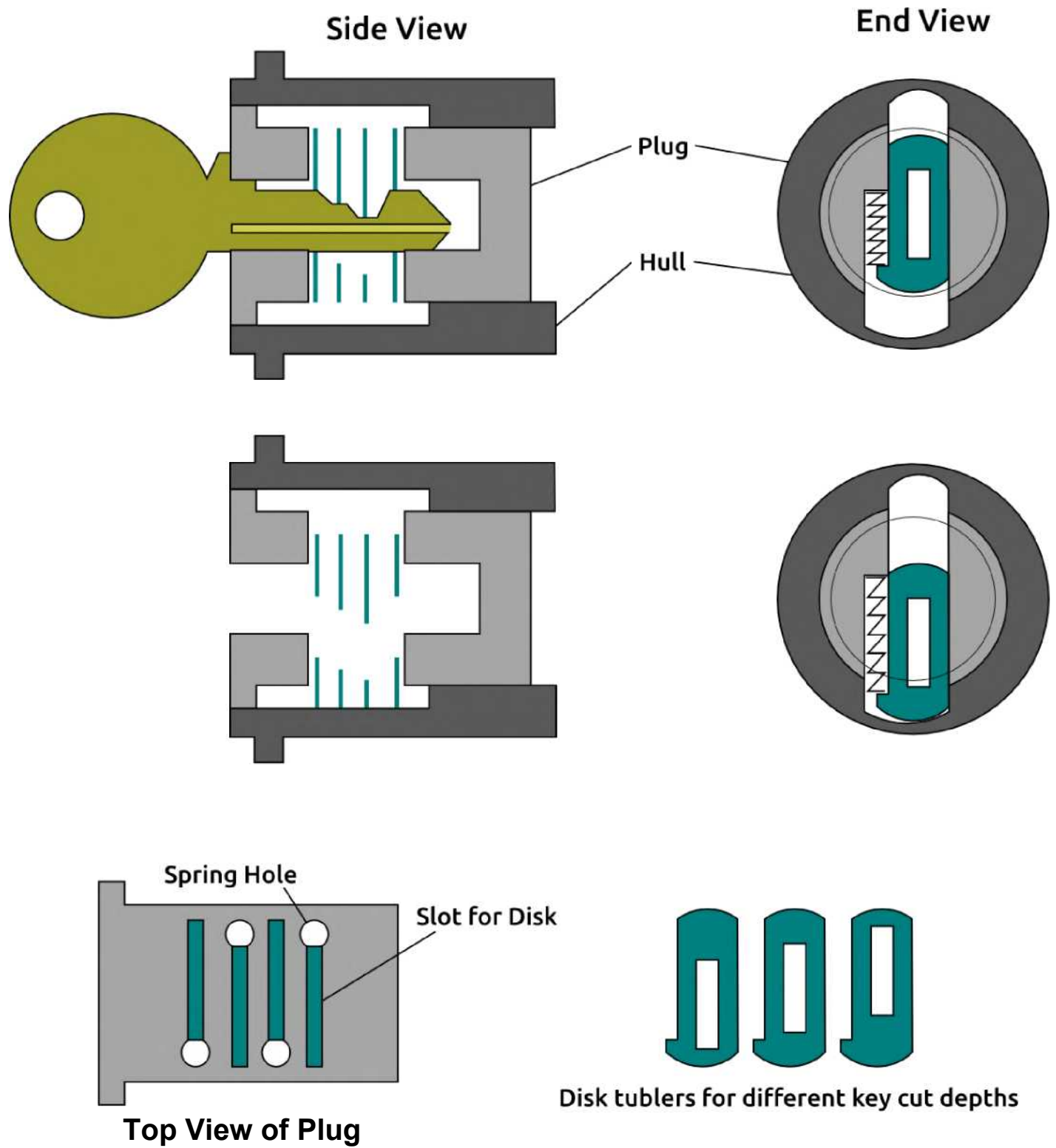
Figure 9.10: Workings of a disk tumber lock
