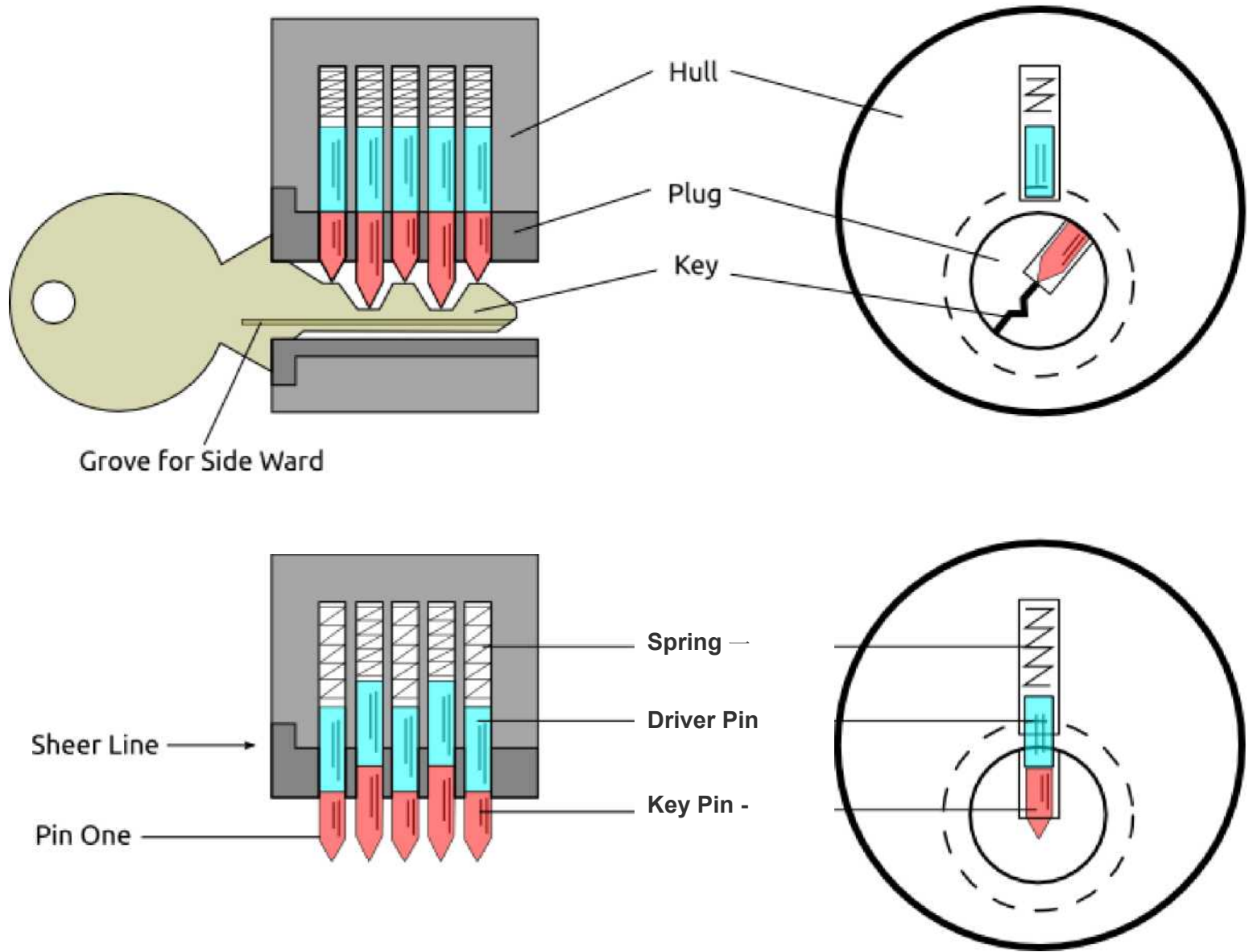
Figure 2.1: Workings of pin tumbler locks
