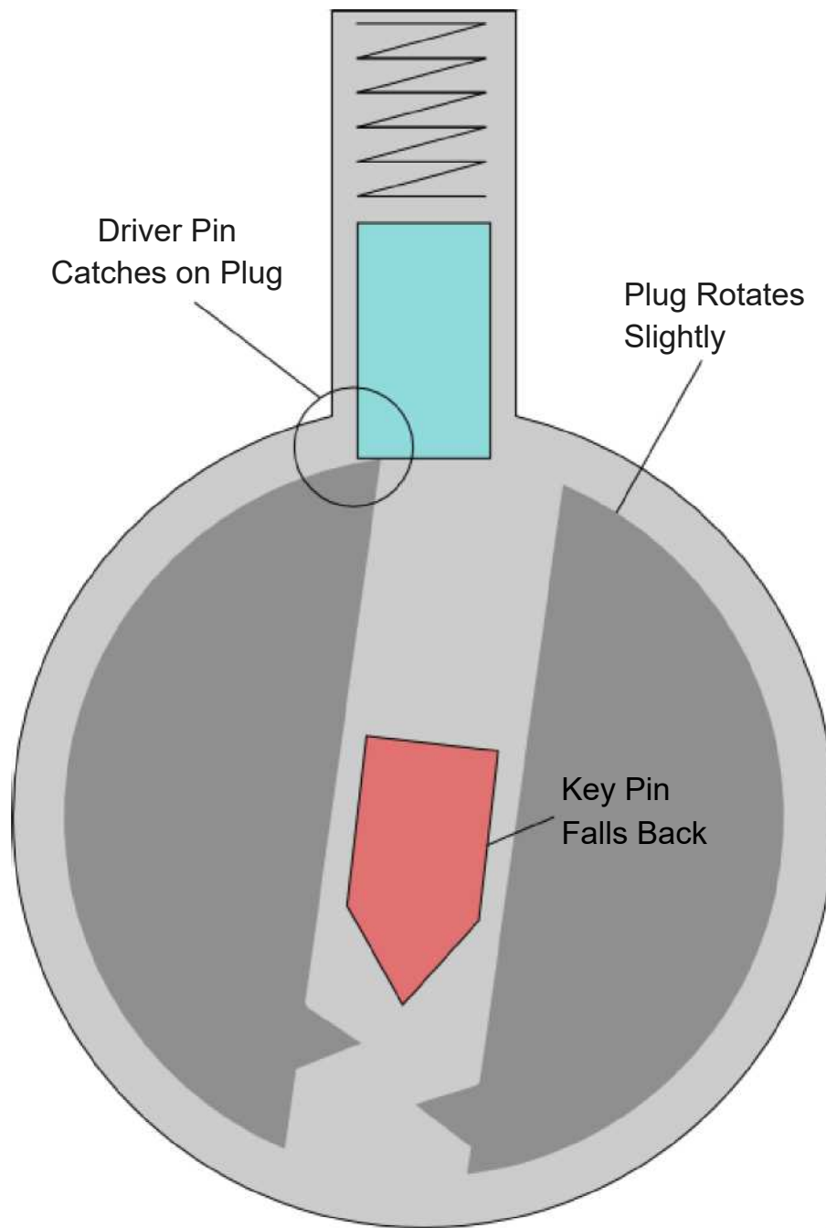
Figure 6.1: Driver pin catches on plug
