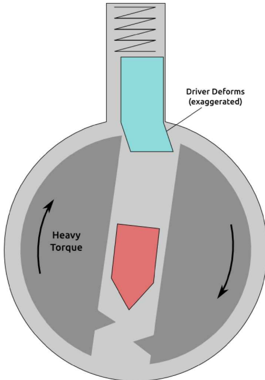
Figure 9.2: Driver pin false set by elastic deformation
