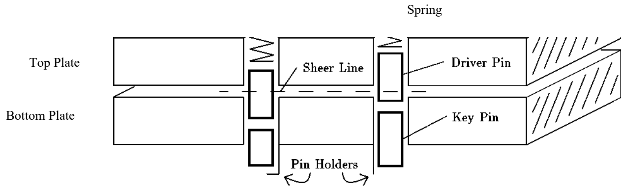
Figure 3.1: Flatland model of a lock
