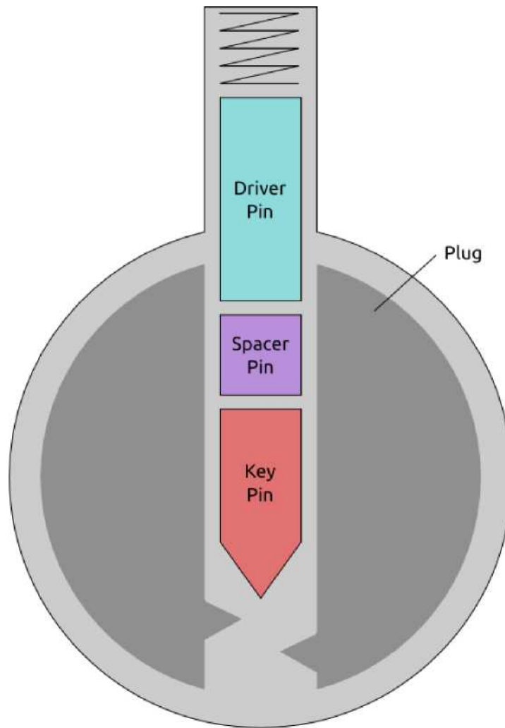
Figure 9.8: Spacer pins for master keying
